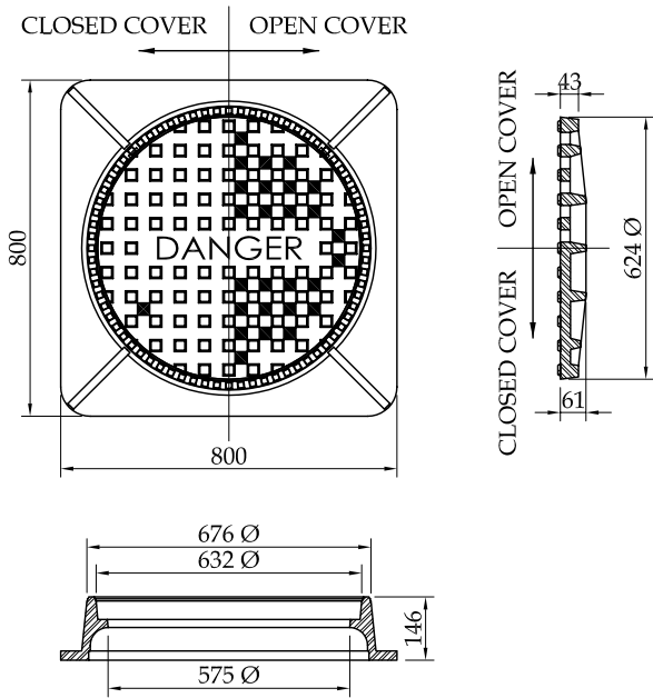
Maintenance Hole Frame & Cover OPSD 401.010 - Type "A" & "B"
