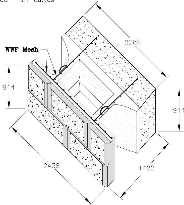
STONE STRONG 24-56 ME - CHISELED GRANITE FACE
