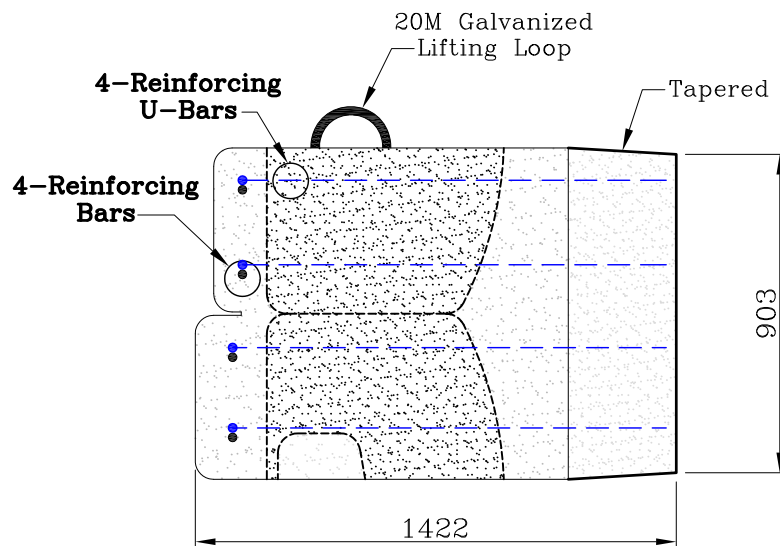
STONE STRONG 24-56 ME - SIDE VIEW
