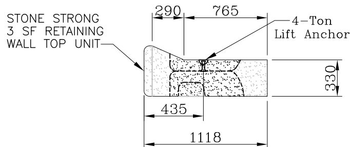
STONE STRONG 3-44 - SIDE VIEW
