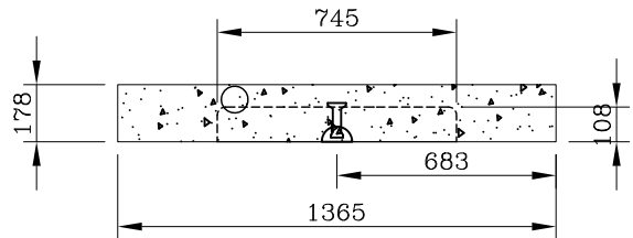
STONE STRONG CAP STEP - END VIEW
