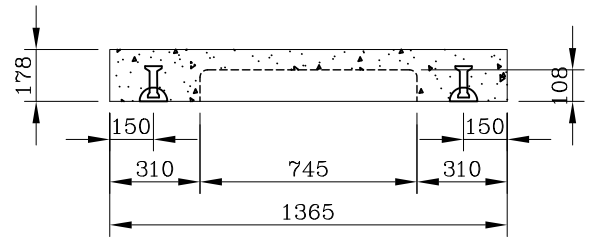
STONE STRONG CAP STEP - SIDE VIEW
