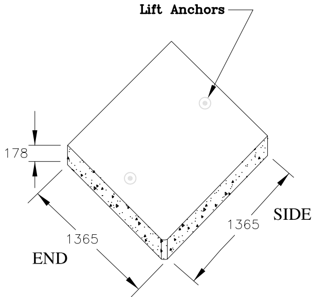
STONE STRONG CAP STEP CHISELED GRANITE FACE
