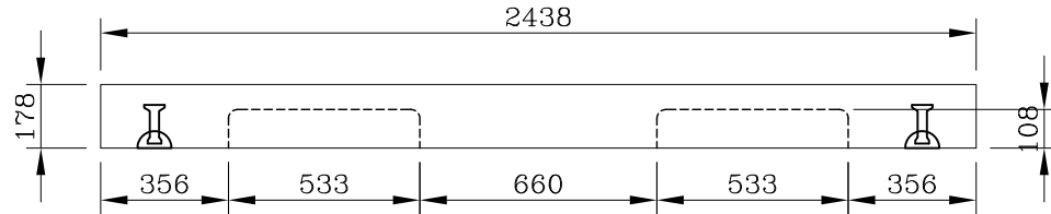
STONE STRONG CAP STEP 8' - SIDE VIEW
