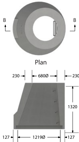
Section B-B
