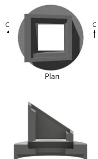
Section C-C
