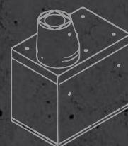
Ditch Inlet Flat Cap (mass - 742 kg + 1133 kg/m)
