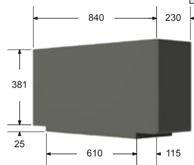
Beam Detail
