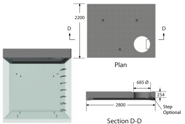
Flat Cap
