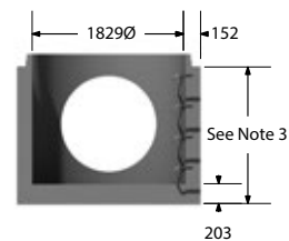
Section C-C
